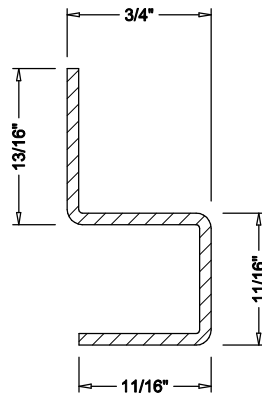
HORIZONTAL MASONRY FASTENER - DETAIL
