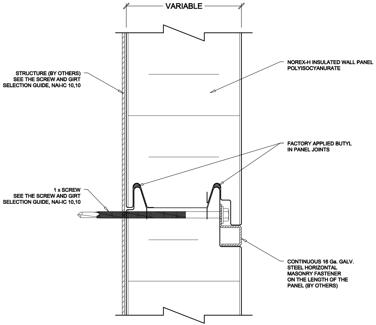
SECTION AT THE GIRT
