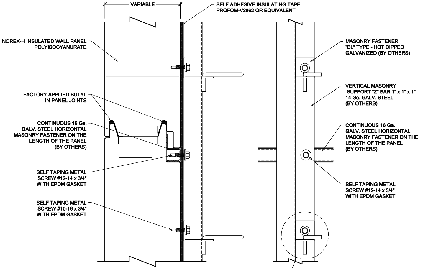
SECTION VIEW OF THE MASONRY SUPPORT "Z" BAR
