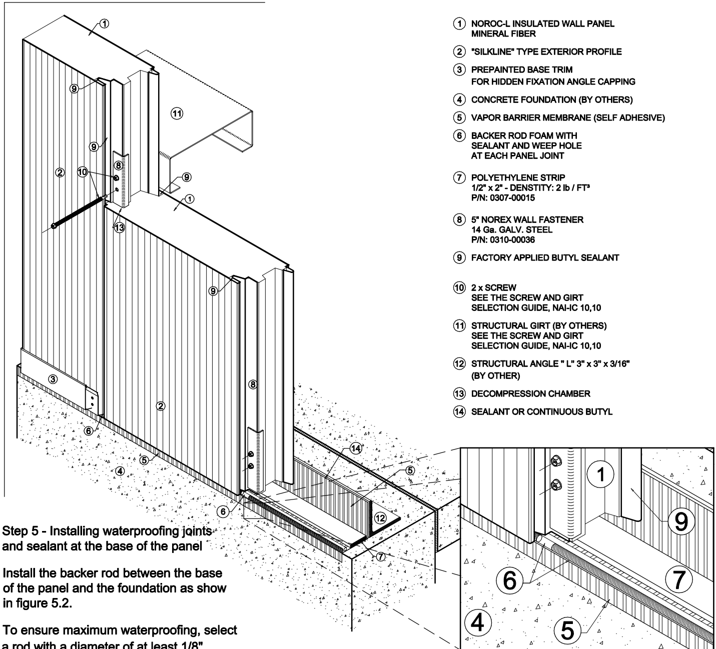
Figure 5.2: Panel Base Detail
