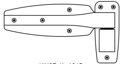
HINGE K-1245 ACCESS DOOR (24" TO 43" WIDE) FLUSH 0313-00006 OFFSET 0313-00007
