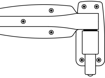
SPRING ASSISTED HINGE K-1248 ACCESS DOOR (24" TO 43" WIDE) 0313-00009/0313-00010
